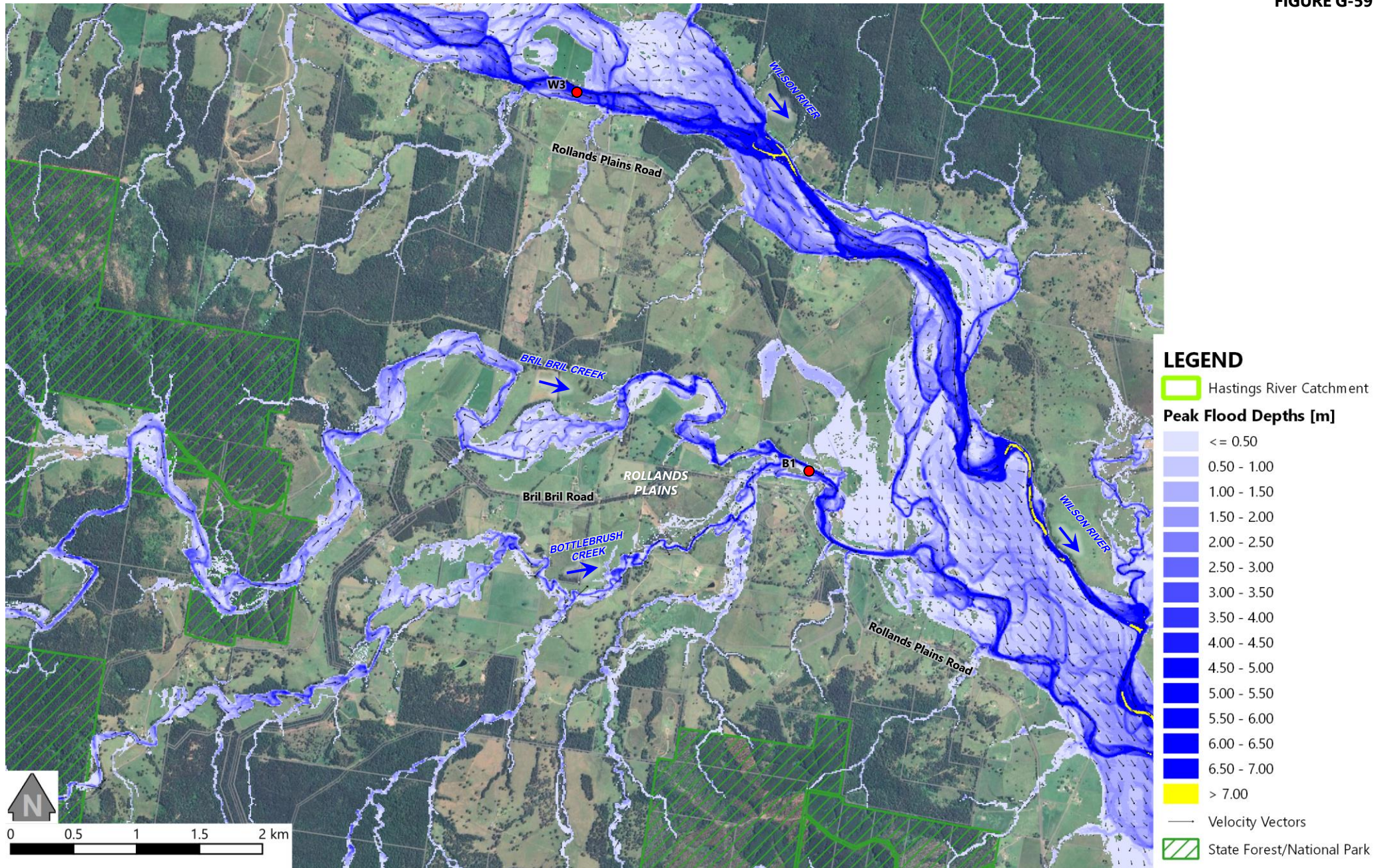
PREDICTED FLOOD DEPTHS AT THE PEAK OF THE DESIGN 1% AEP FLOOD (EXTENT 9 OF 10)
