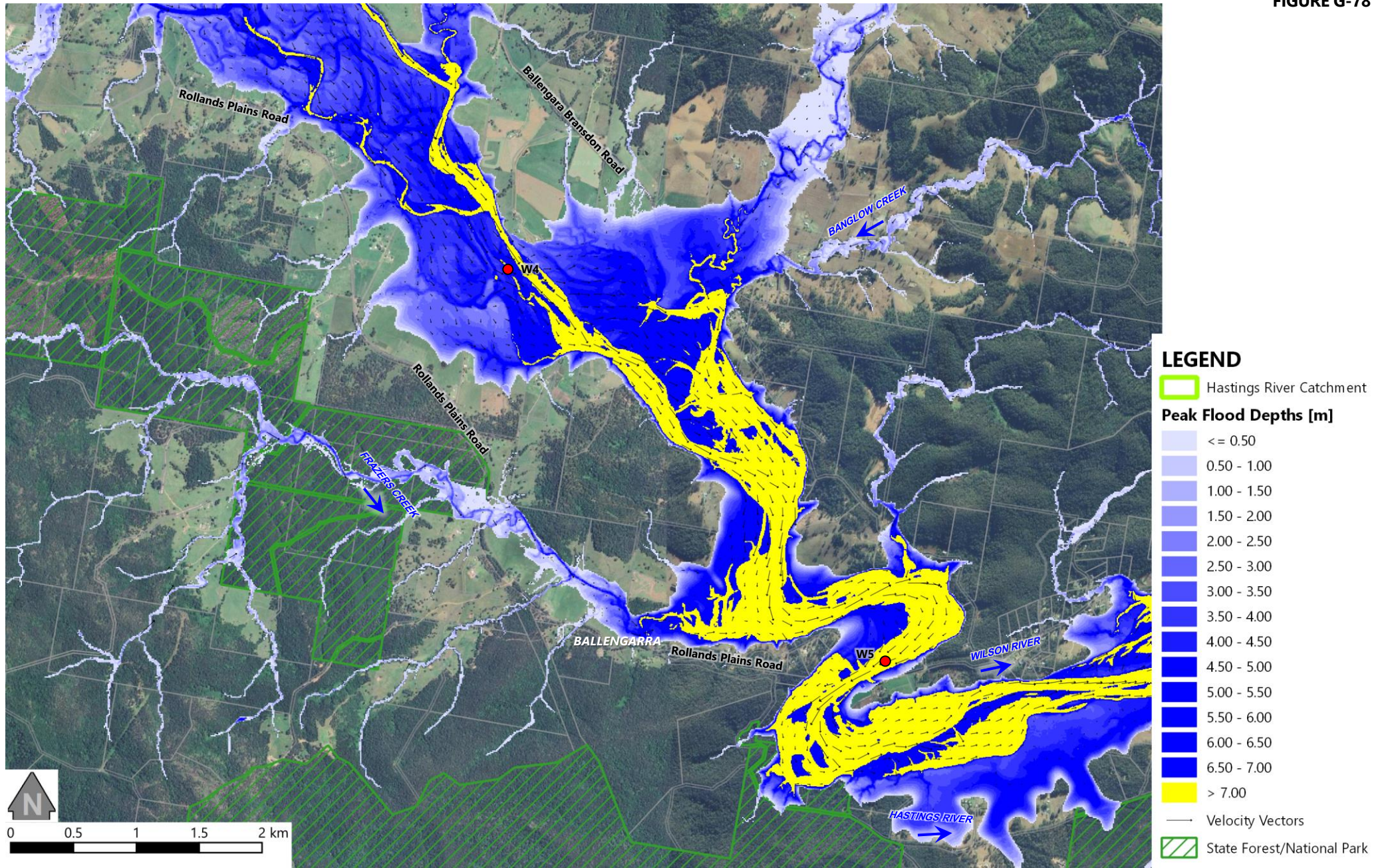
PREDICTED FLOOD DEPTHS AT THE PEAK OF THE DESIGN PMF (EXTENT 8 OF 10)
