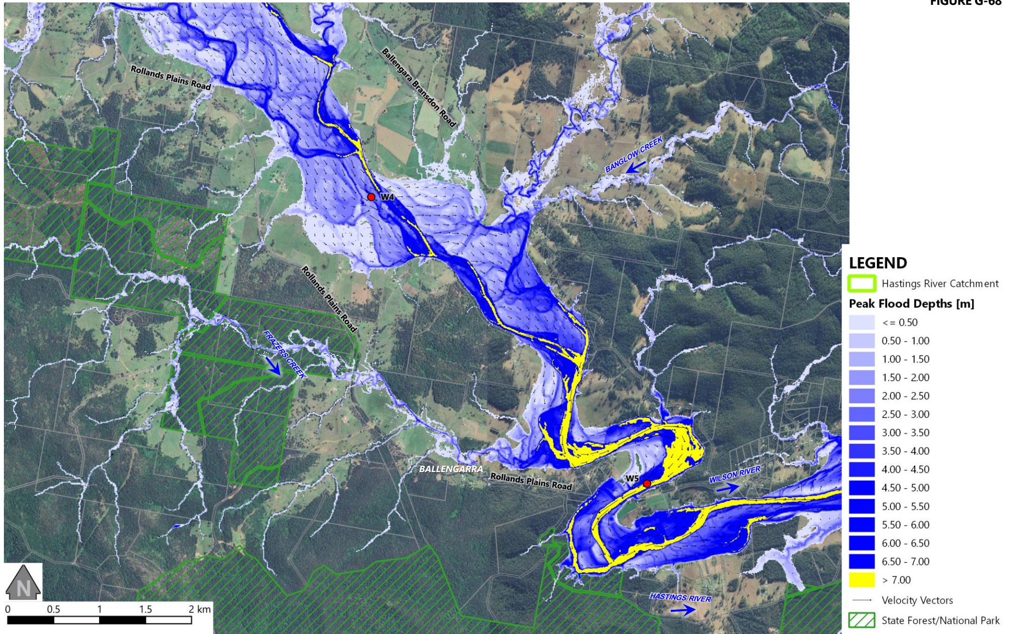
PREDICTED FLOOD DEPTHS AT THE PEAK OF THE DESIGN 1% CC AEP FLOOD (EXTENT 8 OF 10)
