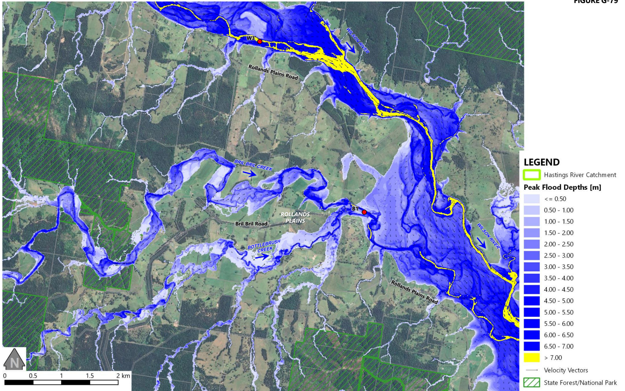
PREDICTED FLOOD DEPTHS AT THE PEAK OF THE DESIGN PMF (EXTENT 9 OF 10)
